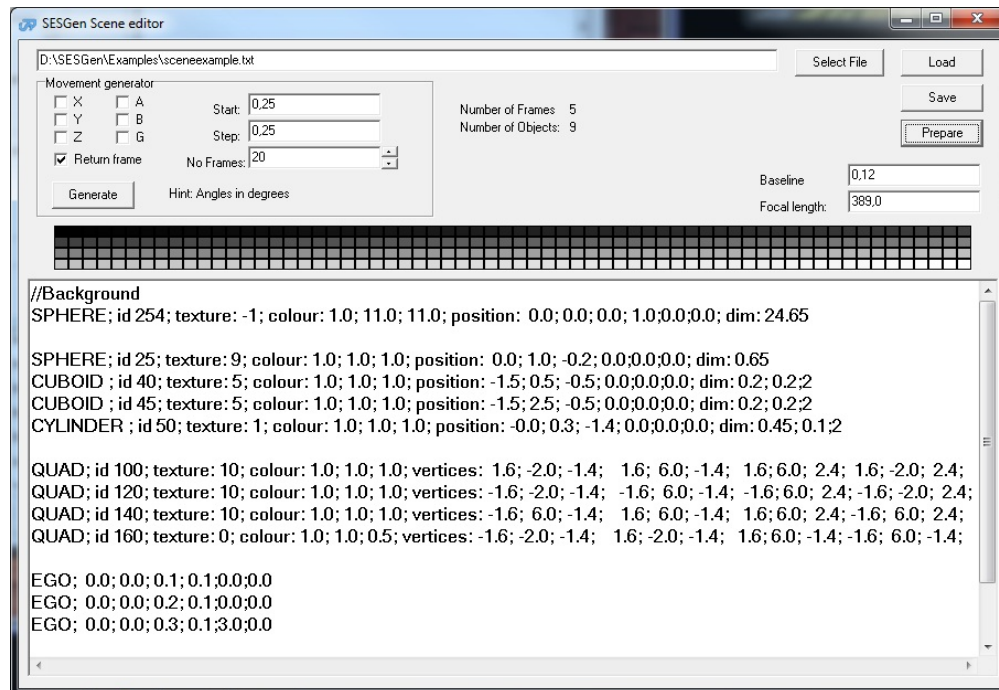
Figure 3: Editor Window
